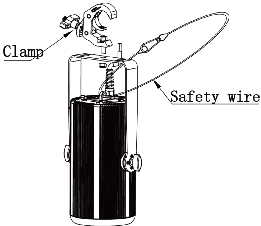
Hanging layout
